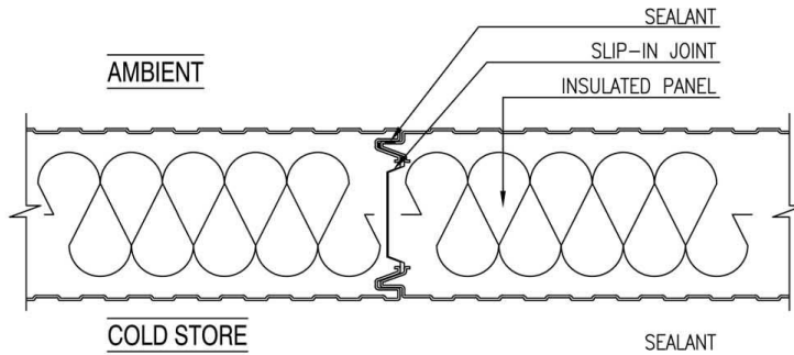
SLIP JOINT WALL/WALL DETAIL SCALE 1:5
