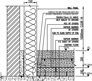
FLOOR/WALL DETAIL SCALE 1:5
