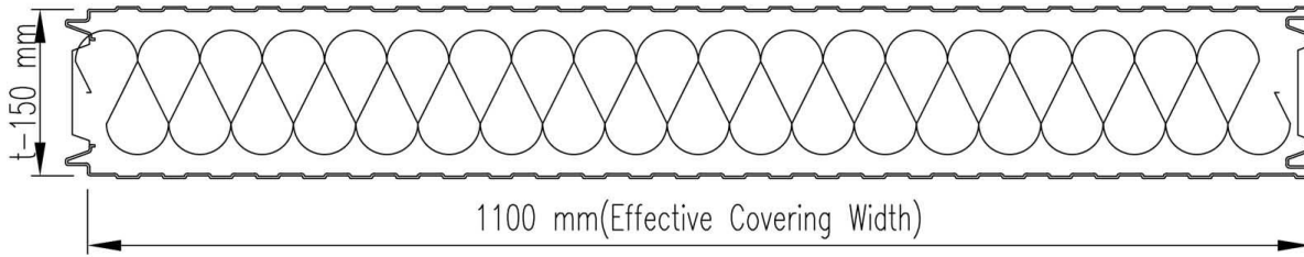
SLIP JOINT PANEL SECTION SCALE 1:5
