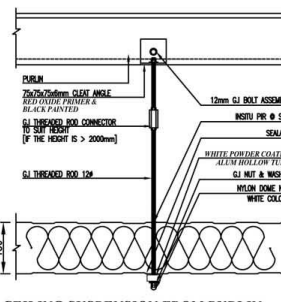
CEILING SUSPENSION FROM PURLIN SCALE 1:5
