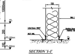
SECTION 'I-I' SCALE 1:5
