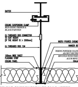
CEILING SUSPENSION FROM RAFTER SCALE 1:5
